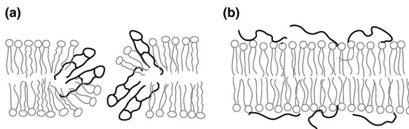
Fig. 9. Models of the different interactions between PG-1 mutants and anionic lipid bilayers. (a) [\Delta_{4,18} G_{10}] PG-1 has a well defined \beta -hairpin conformation, disrupts the lamellar structure of the lipid membrane, and likely inserts into the bilayer. (b) [A_{6,8,13,15}] PG-1 has a random coil conformation in solution, does not cause significant membrane disorder, and likely binds to the surface of the membrane.
