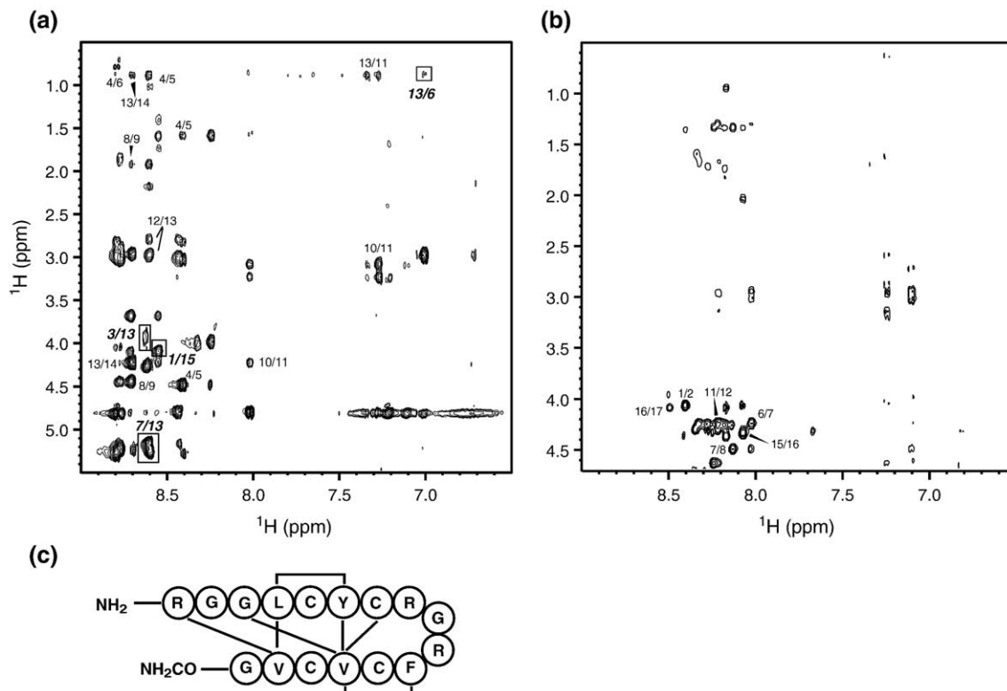
Fig. 8. (a) 2D NOESY spectrum of [ \Delta_{4,18} G _{10} ] PG-1 with a mixing time of 300 ms. Cross-strand NOE peaks are boxed. (b) 2D NOESY spectrum of [ A_{6,8,13,15} ] PG-1 with a mixing time of 300 ms. (c) Schematic representation of [ \Delta_{4,18} G _{10} ] PG-1, in which the observed non-sequential NOEs are drawn.
