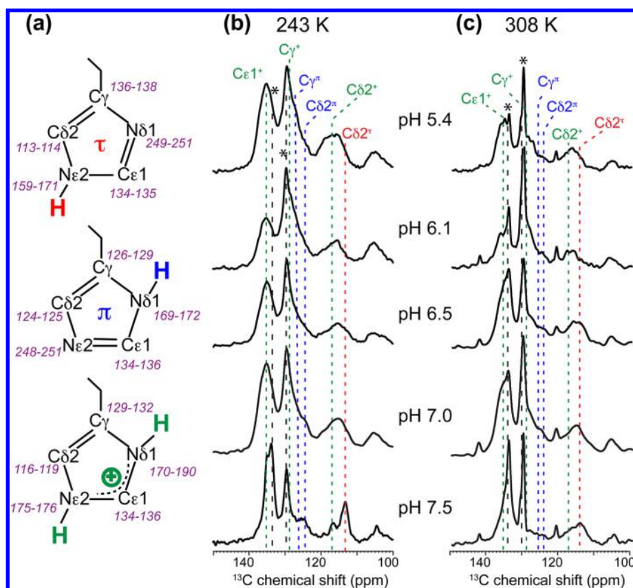
Figure 2. (a) Chemical structures of the three forms of histidine and their characteristic chemical shift ranges. (b and c) Aromatic region of the ^{13}\text{C} CP-MAS spectra of His37 in VM+ bound M2(21–97) from pH 7.5 to 5.4. Peak assignments are shown in red for the \tau tautomer, blue for the \pi tautomer, and green for cationic histidine. Asterisks indicate the lipid natural-abundance ^{13}\text{C} peaks. (b) 243 K spectra. (c) 308 K spectra.
