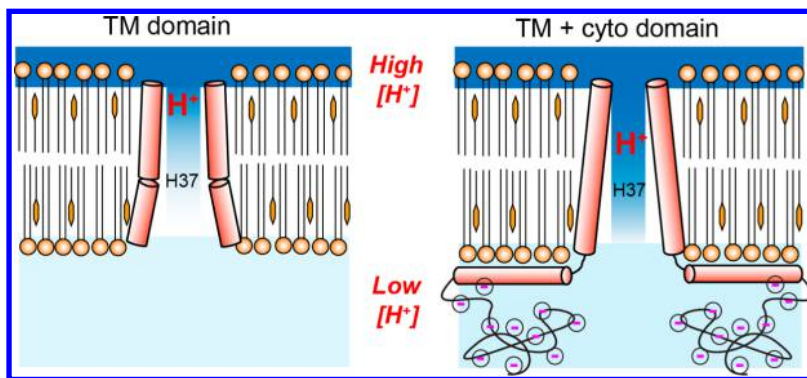
Figure 9. Schematic model of His37-mediated proton conduction in cytoplasmic-containing M2. The cytoplasmic domain, which contains a large number of acidic residues, facilitates proton conduction through electrostatic effects increasing the His37 pK_a 's compared to the TM construct. The darker blue gradient on the right depicts higher proton concentrations in the channel. The His37 backbone is more \alpha -helical in the longer M2 construct, which may result from electrostatic repulsion among the four negatively charged cytoplasmic domains. For clarity, only two of the four molecules of the tetrameric channel are depicted.
